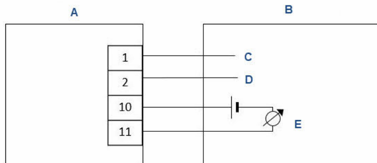
Figure 2-9: Sink four-wire
