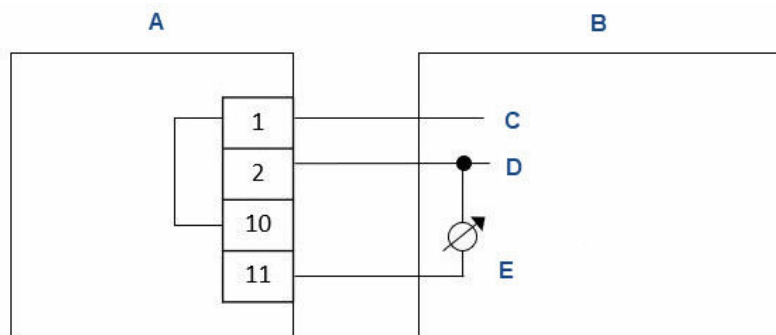
Figure 2-10: Source three-wire
