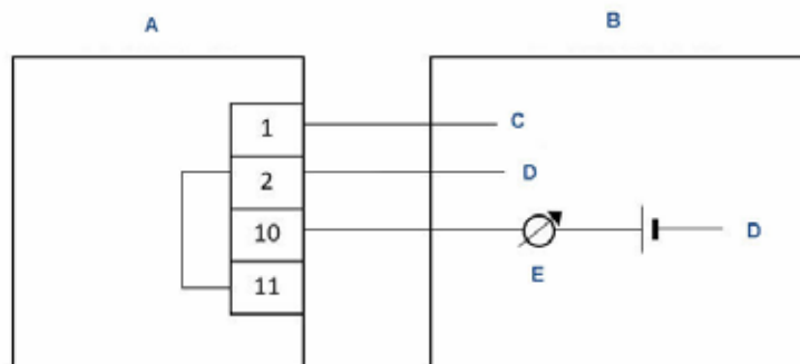
Figure 2-8: Non-isolated sink (three wires)
