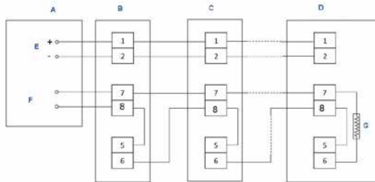
Figure 2-7: Typical wiring for four-wire controllers
