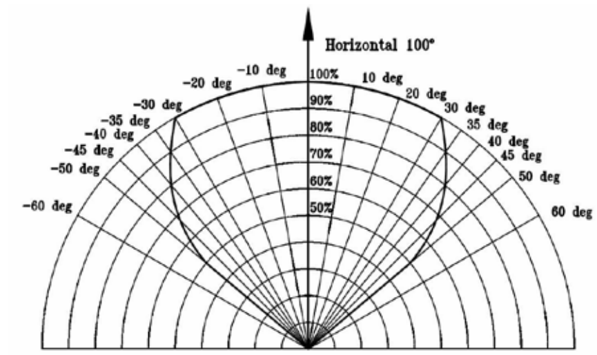
Figure 2-1: Horizontal field of view for SharpEye 40/40C-I, C-LB, C-L4B, D-I, D-LB, and D-L4B
